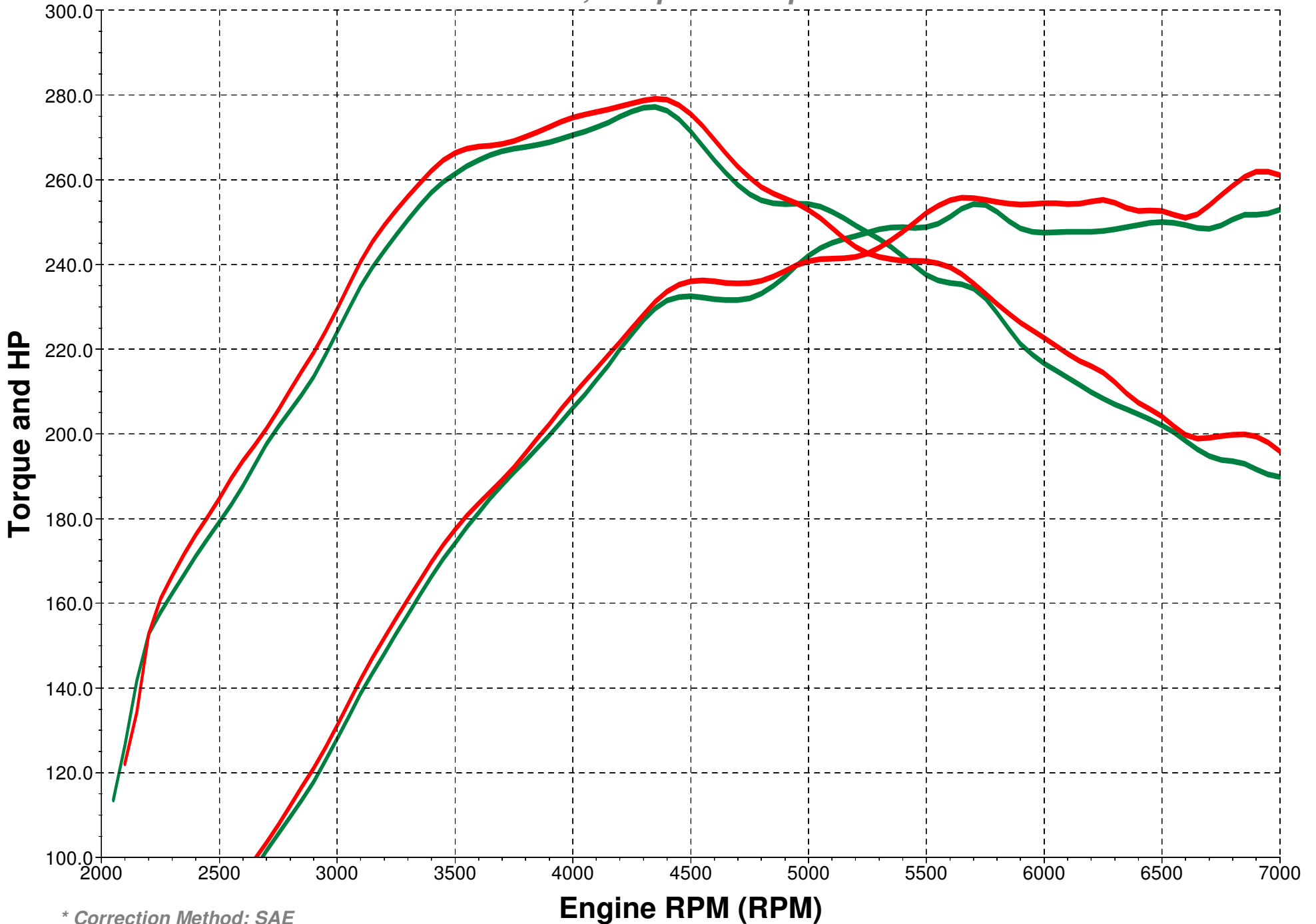
A/F Ratio, Torque and Hp vs. RPM
